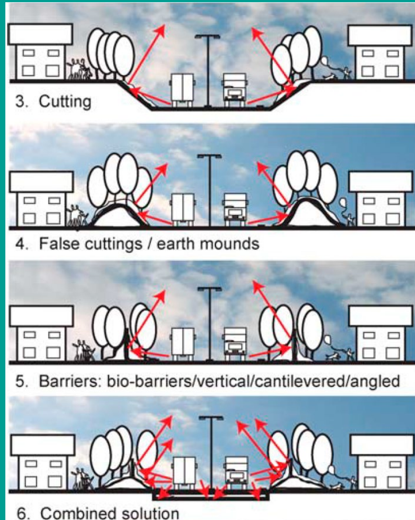
Bild: "Environmental Noise Barriers: A Guide to their Acoustic and Visual Design" 2nd Ed., Dr Benz Kotzen, Greenwich University, ISBN O-203-93138-6, p. 34, 2009
