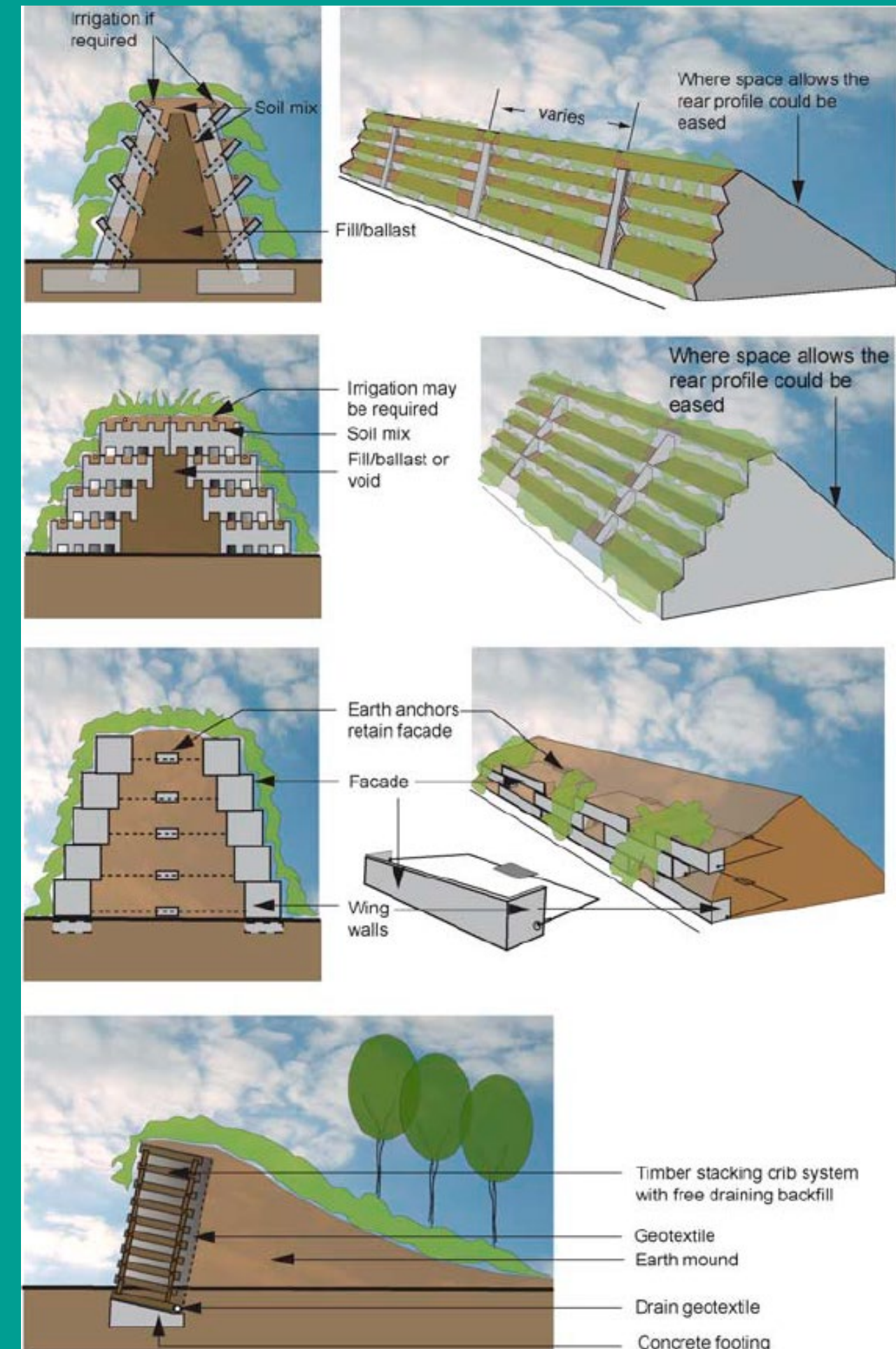
Bild: "Environmental Noise Barriers: A Guide to their Acoustic and Visual Design" 2nd Ed., Dr Benz Kotzen, Greenwich University, ISBN O-203-93138-6, p. 180, 2009
